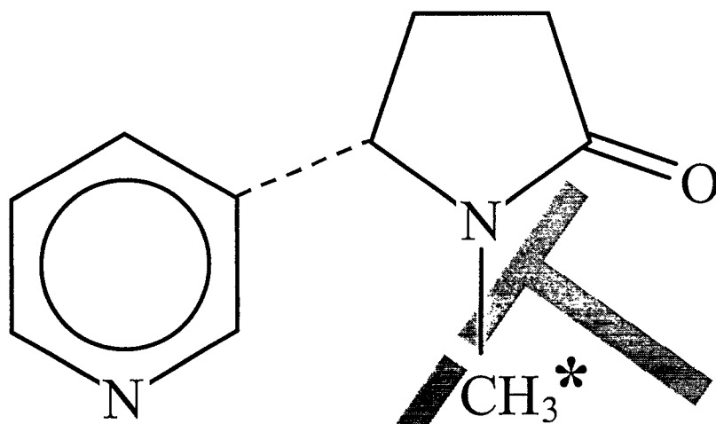
Cotinine
