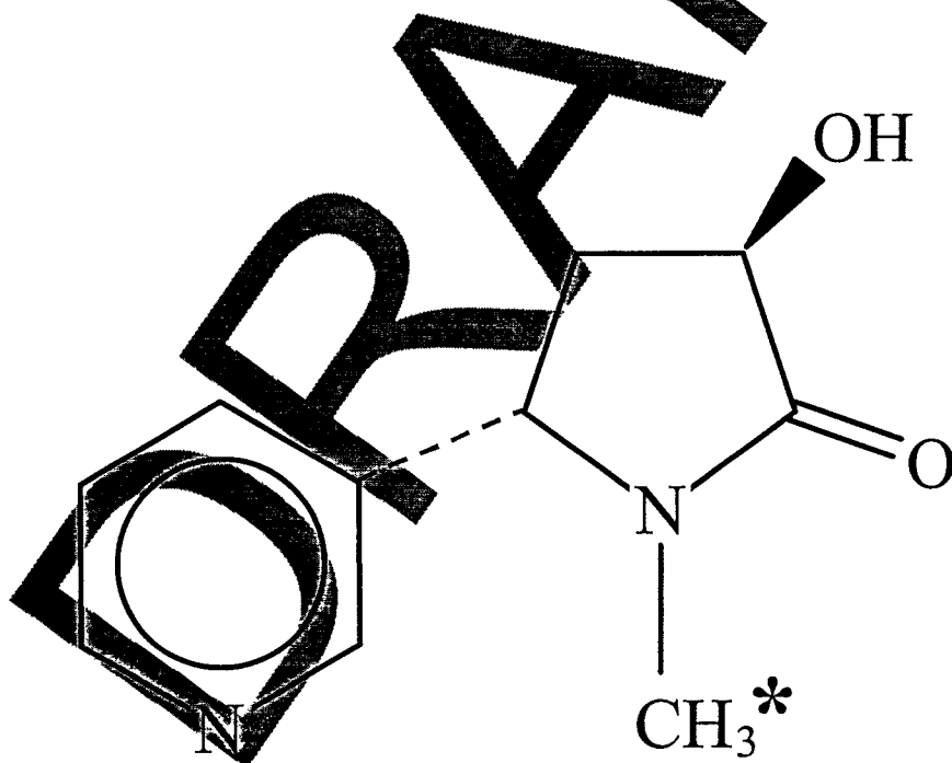
3-Hydroxycotinine
